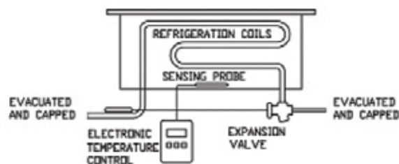
RCP7XXX HRCF7XXX 'NC' REFRIGERATION SCHEMATIC
